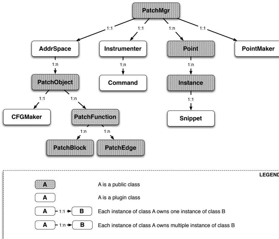
Figure 1: Object Ownership
